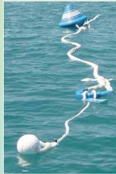
Mooring buoy, pick-up tag and pick-up line
